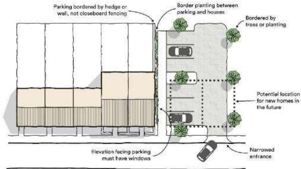
Peripheral parking forming a courtyard to the side of houses, with potential future semi-detached homes shown in a dashed line
