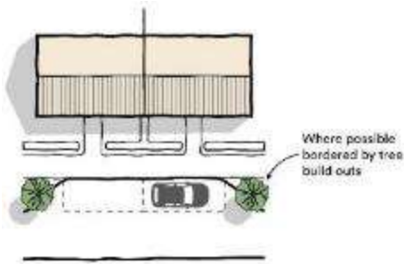
Formal on-street parking, which can be bordered by tree build outs
